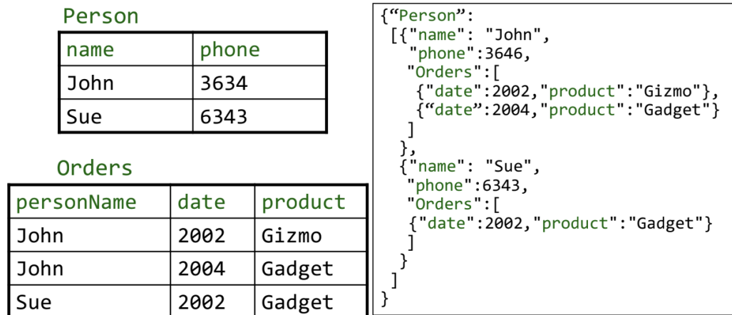
Figure 6: A JSON representation of relational tables
